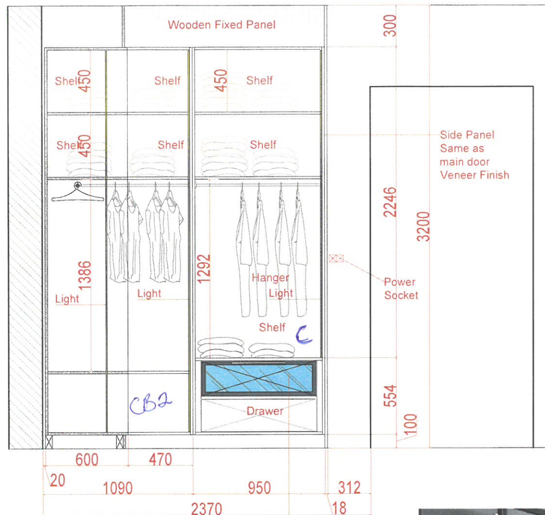
Elevation- C Details
