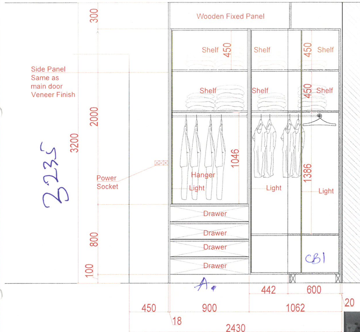
Elevation- A Details
