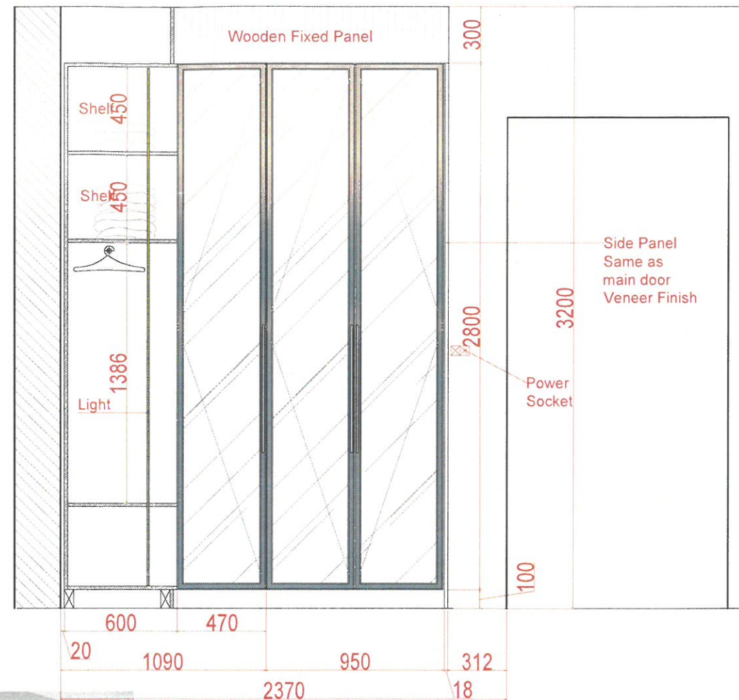
Elevation- C Details with Doors
