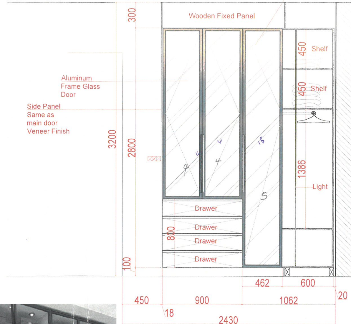
Elevation- A Details with Doors
