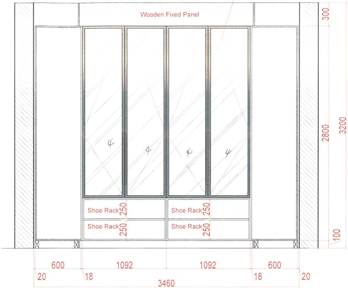
Elevation- B Details with Door
