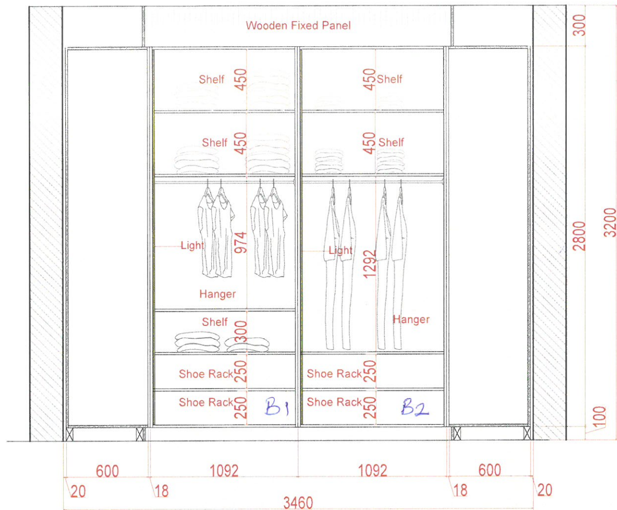
Elevation- B Details
